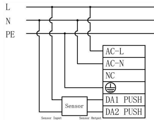
Wiring diagram of corridor dimming
